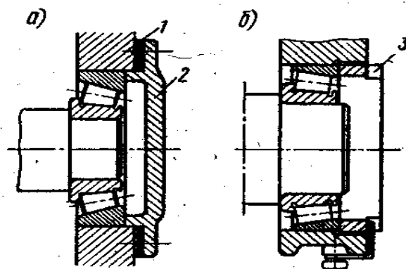
17.8-rasm. Konussimon rolikli podshipnikda tirqishni sozlash usullari
