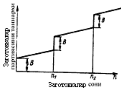
11.2-rasm. Qo'shimcha jihoz qo'llash natijasida tannarx C ning o'zgarishi
