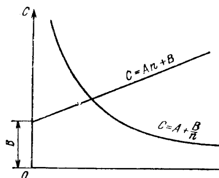
10.1-rasm. Ishlov beriladigan zagotovkalar sonini ortishi bilan tannarx C ning o'zgarishi
