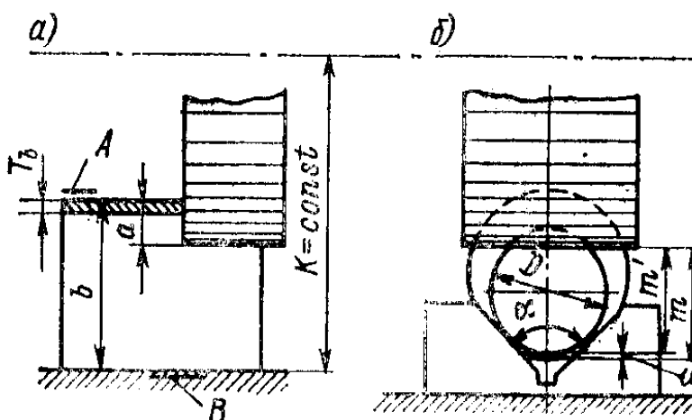
2.13-rasm. Bazalash hatoligi \omega_{\Delta} = \omega_{\phi} ning kelib chiqishi
