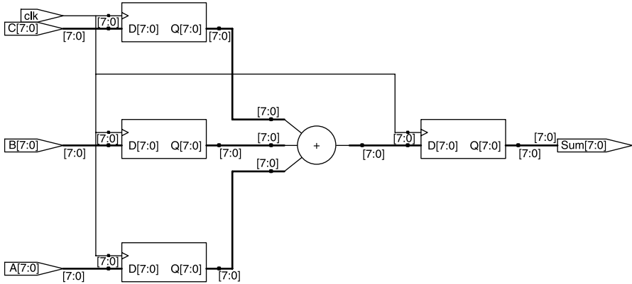
Figure 1.9 Registered adder.
