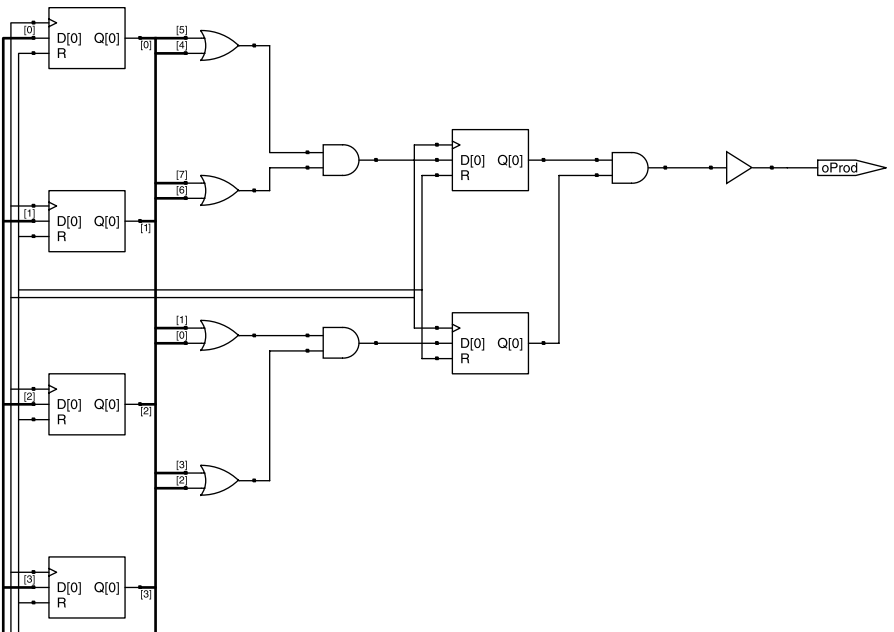
Figure 14.10 Balanced logic.
