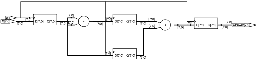
Figure 1.2 Pipelined implementation.
