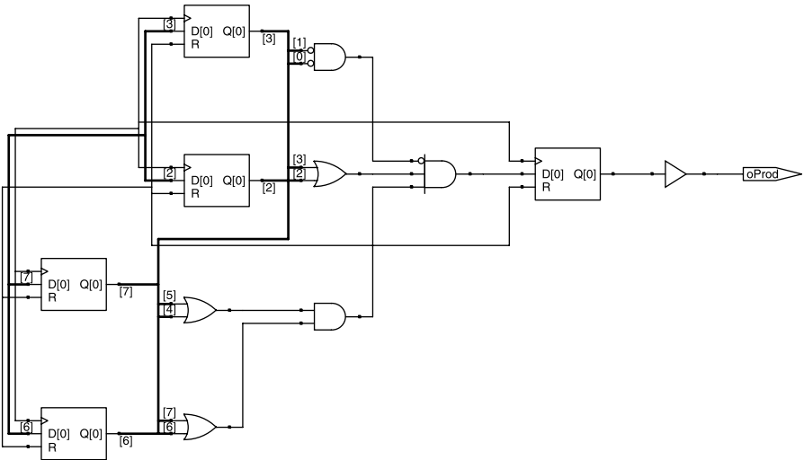
Figure 14.9 Imbalanced logic.
