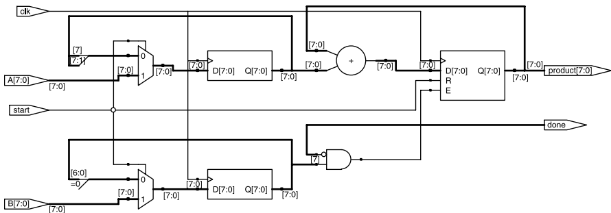
Figure 2.1 Shift/add multiplier.
