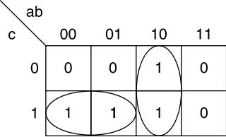
Figure 10.12 Identifying the static-1 hazard.
