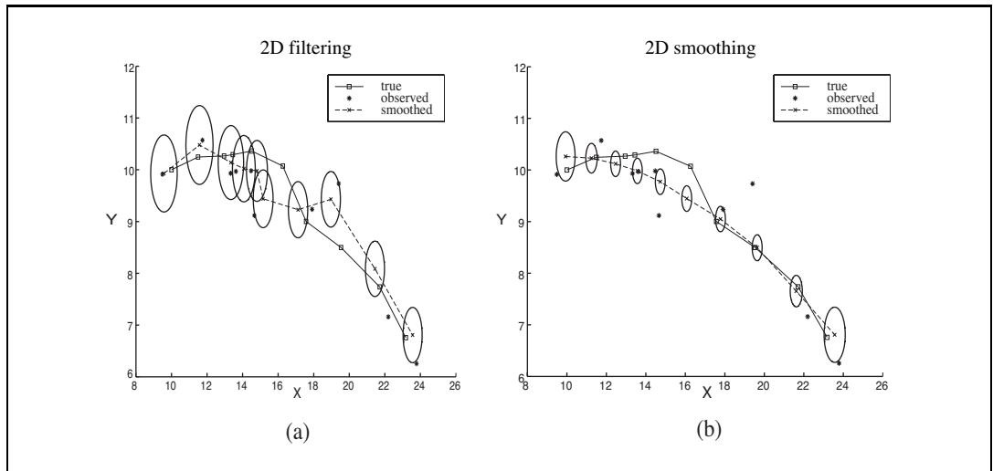
Figure 15.11 (a) Results of Kalman filtering for an object moving on the X - Y plane, showing the true trajectory (left to right), a series of noisy observations, and the trajectory estimated by Kalman filtering. Variance in the position estimate is indicated by the ovals. (b) The results of Kalman smoothing for the same observation sequence.
