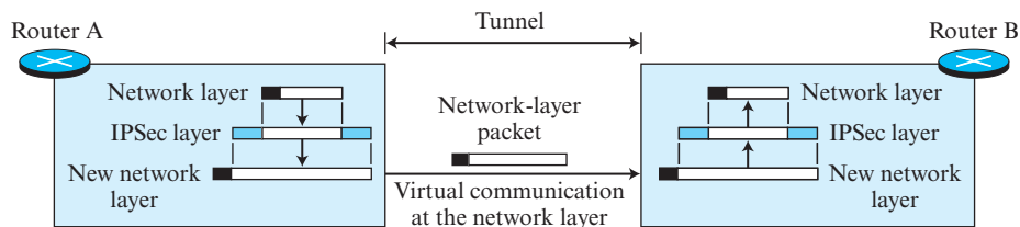
Figure 10.49 Tunnel mode in action
