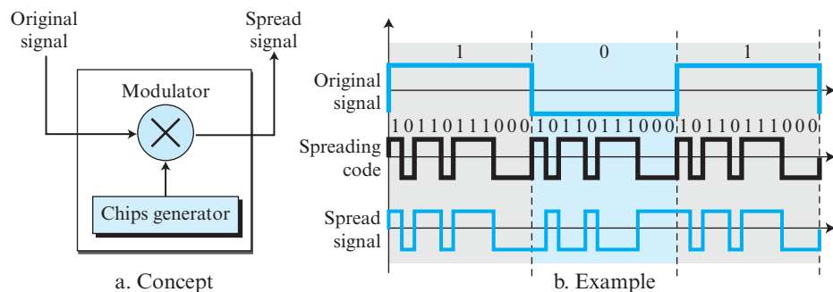
Figure 7.57 DSSS
