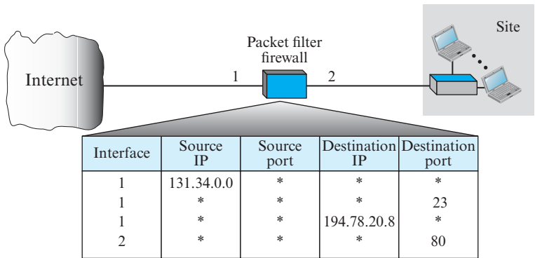
Figure 10.61 Packet-filter firewall
