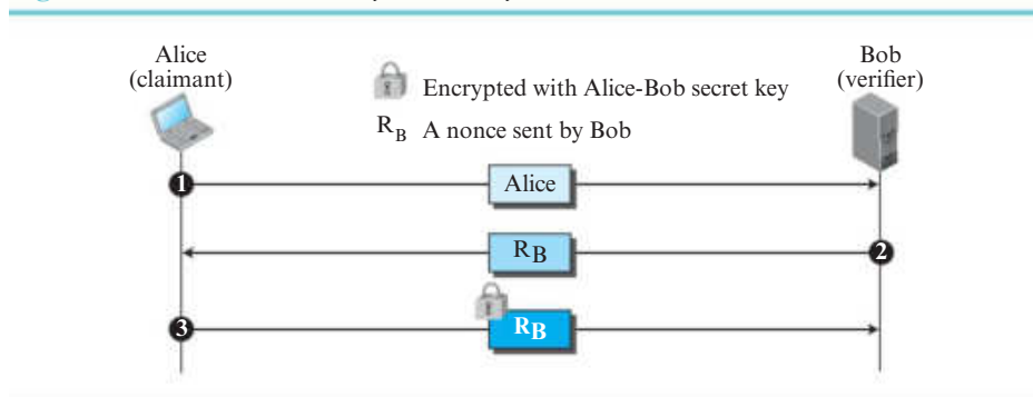
Figure 10.22 Unidirectional, symmetric-key authentication
