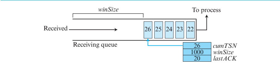
Figure 8.54 Flow control, receiver site
