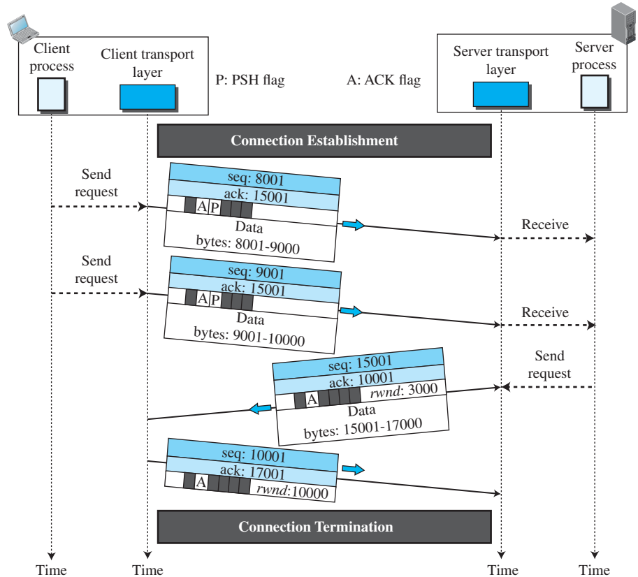
Figure 3.48 Data transfer
