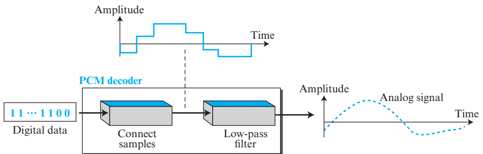
Figure 7.33 Components of a PCM decoder
