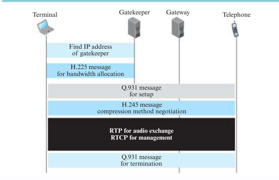
Figure 8.44 H.323 example
