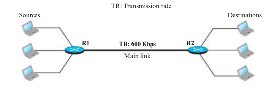
Figure 4.12 Effect of throughput in shared links
