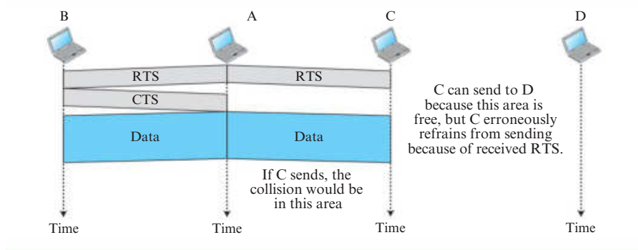
Figure 6.14 Exposed station problem
