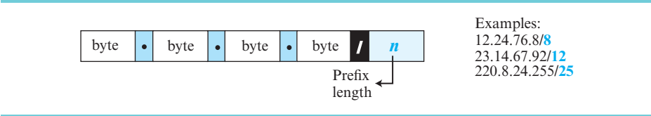
Figure 4.33 Slash notation (CIDR)
