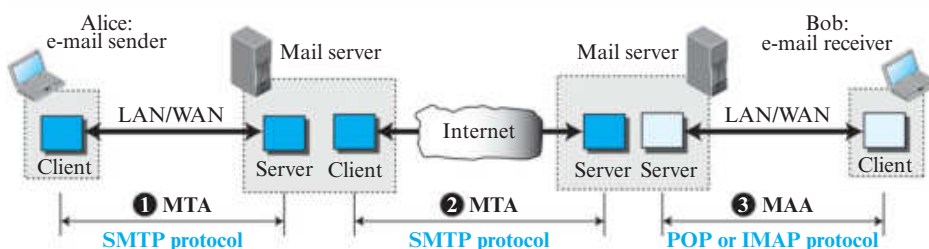
Figure 2.22 Protocols used in electronic mail
