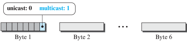
Figure 5.56 Unicast and multicast addresses
