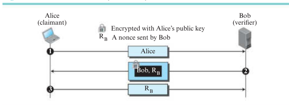
Figure 10.23 Unidirectional, asymmetric-key authentication
