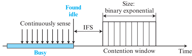
Figure 6.8 Contention window
