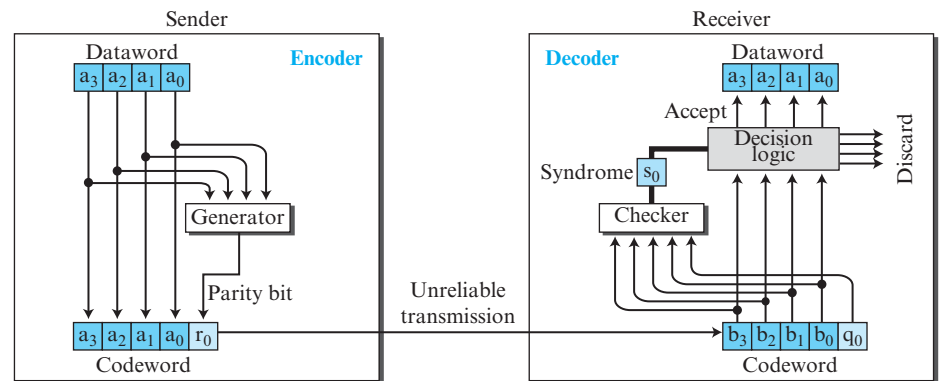
Figure 5.11 Encoder and decoder for simple parity-check code
