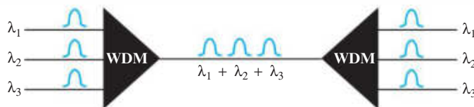
Figure 7.47 Wavelength-division multiplexing
