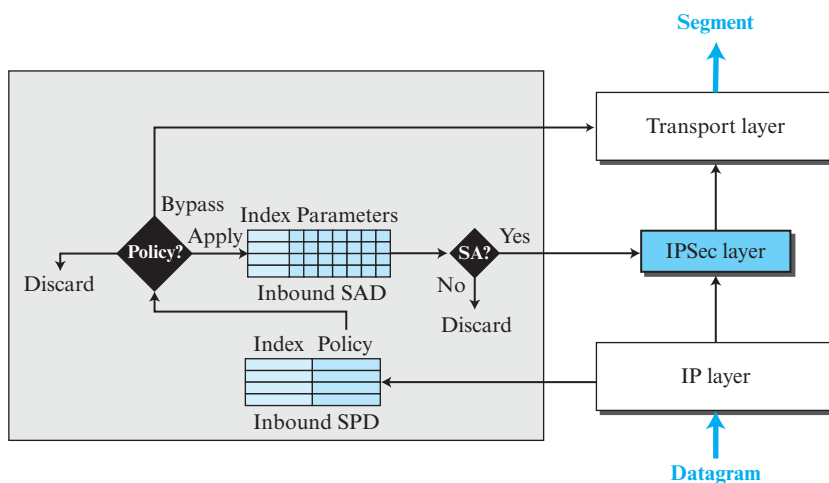
Figure 10.57 Inbound processing
