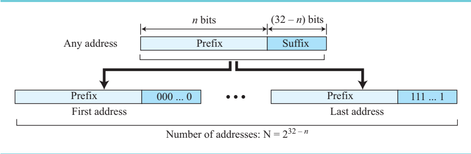
Figure 4.34 Information extraction in classless addressing
