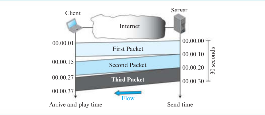
Figure 8.29 Jitter
