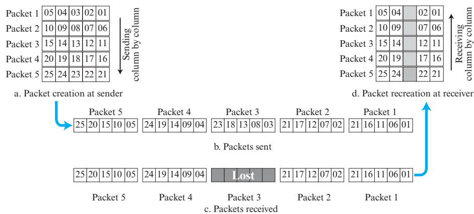
Figure 8.33 Interleaving
