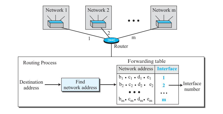
Figure 4.35 Network address
