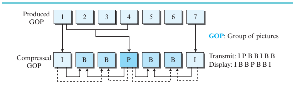
Figure 8.22 MPEG frames
