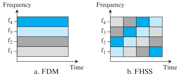
Figure 7.56 Bandwidth sharing
