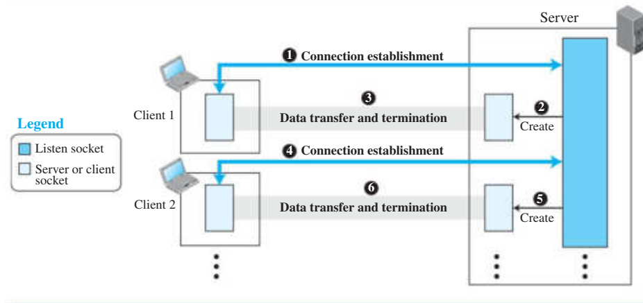
Figure 11.4 ServerSocket and Socket objects in TCP communication
