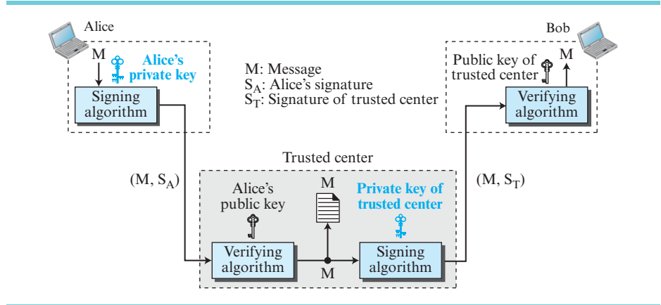
Figure 10.20 Using a trusted center for non-repudiation
