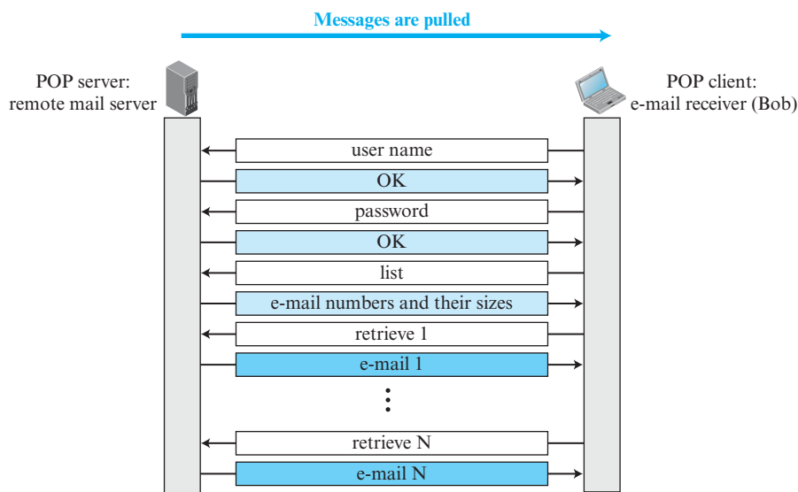
Figure 2.24 POP3
