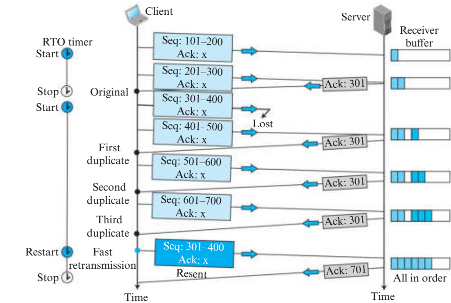
Figure 3.63 Fast retransmission
