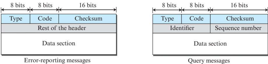
Figure 4.54 General format of ICMP messages
