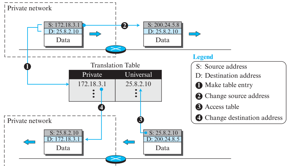
Figure 4.44 Translation
