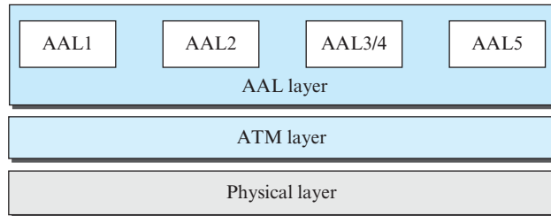
Figure 5.82 ATM layers
