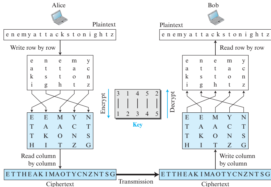
Figure 10.6 Transposition cipher
