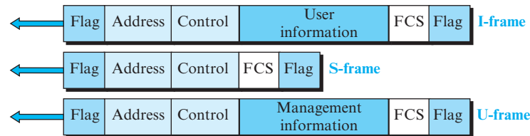
Figure 5.22 HDLC frames
