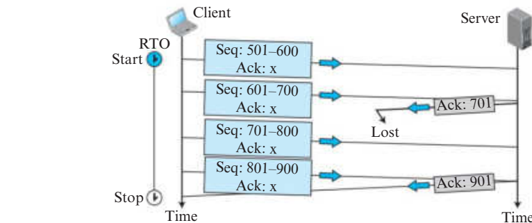
Figure 3.64 Lost acknowledgment
