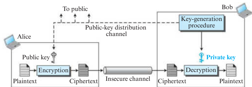
Figure 10.14 General idea of asymmetric-key cryptosystem
