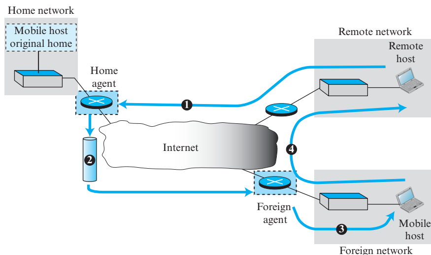
Figure 6.58 Data transfer
