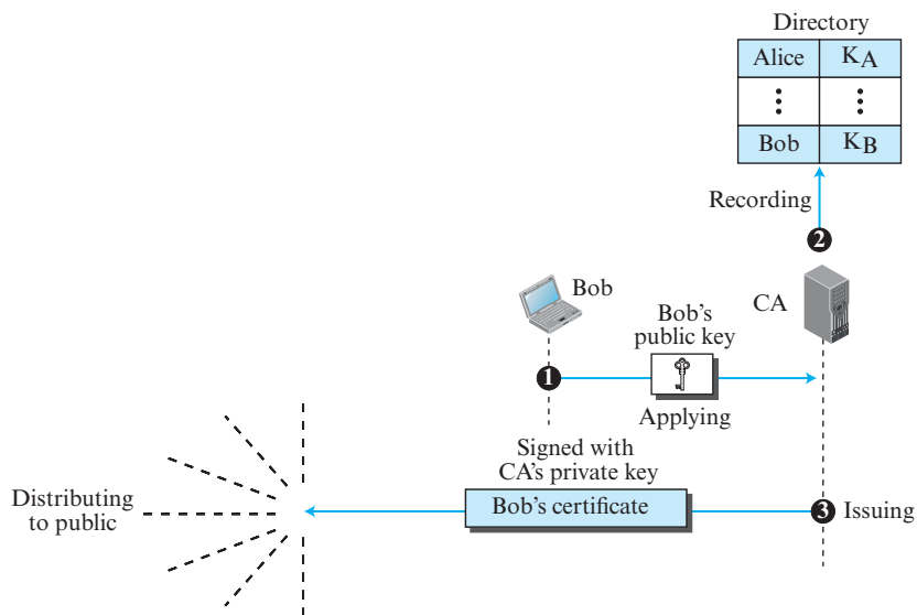
Figure 10.28 Certification authority
