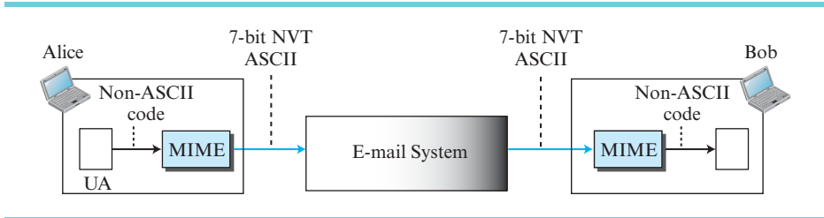
Figure 2.25 MIME
