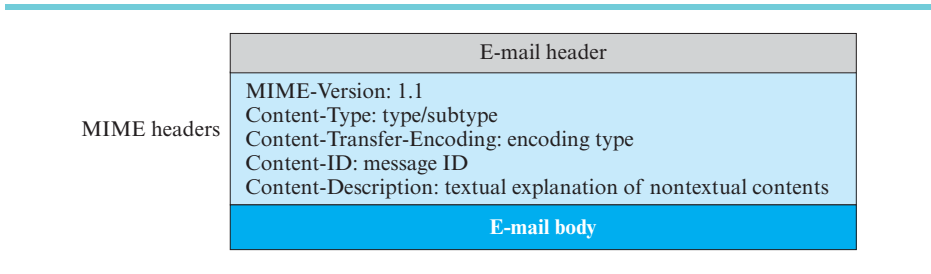
Figure 2.26 MIME header
