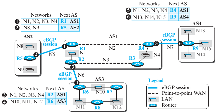
Figure 4.80 eBGP operation
