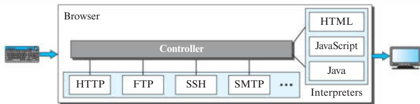
Figure 2.9 Browser
