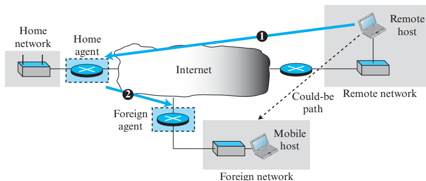
Figure 6.60 Triangle routing
