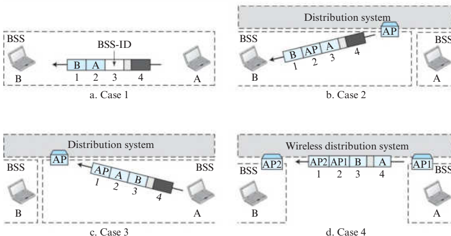
Figure 6.13 Addressing mechanisms
