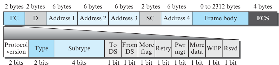
Figure 6.11 Frame format
