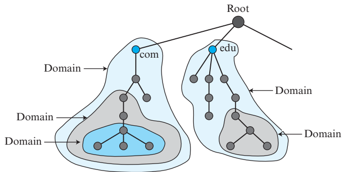
Figure 2.38 Domains
