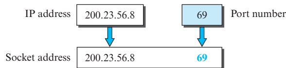
Figure 3.6 Socket address
