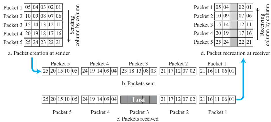
Figure 8.33 Interleaving
