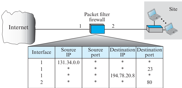
Figure 10.61 Packet-filter firewall
