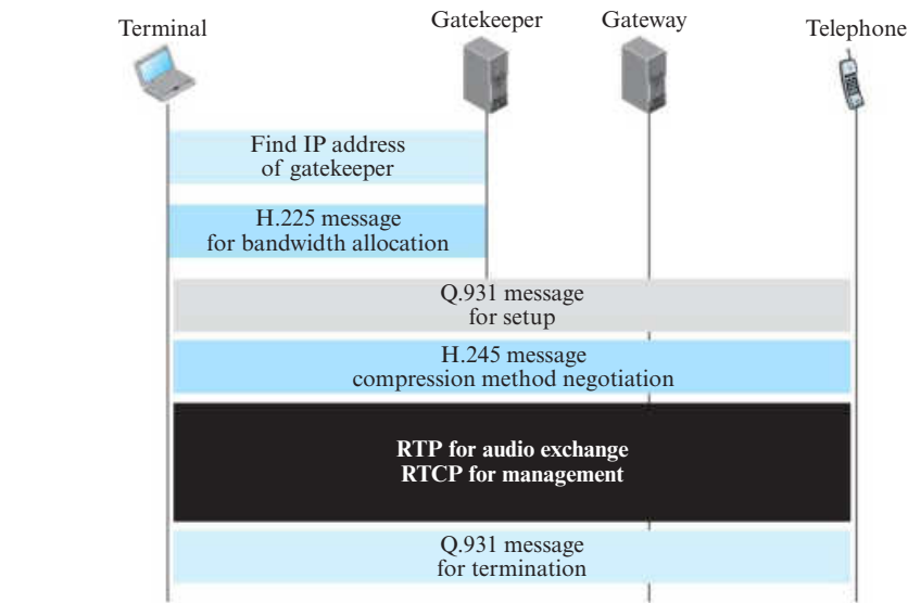
Figure 8.44 H.323 example
