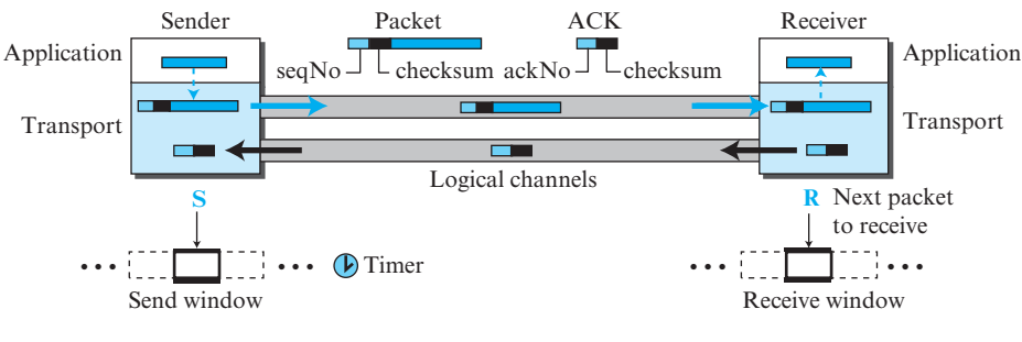
Figure 3.20 Stop-and-Wait protocol
