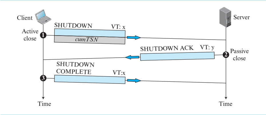
Figure 8.53 Association termination
