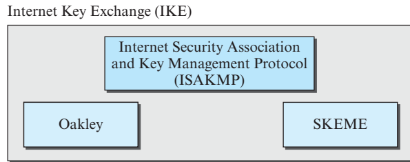
Figure 10.58 IKE components
