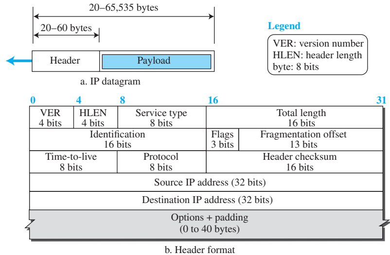
Figure 4.24 IP datagram
