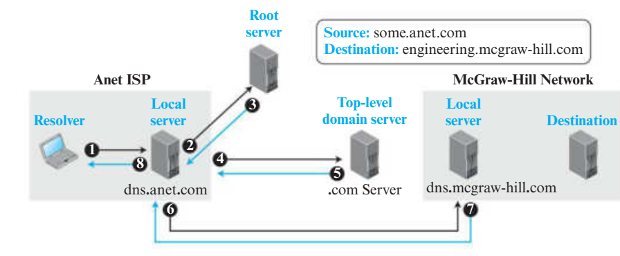
Figure 2.44 Iterative resolution
