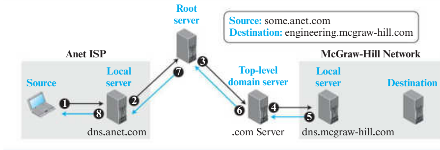
Figure 2.43 Recursive resolution
