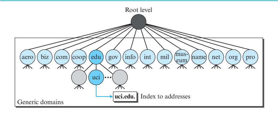
Figure 2.41 Generic domains
