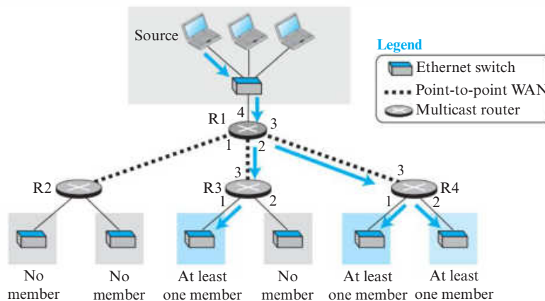
Figure 4.88 Multicasting
