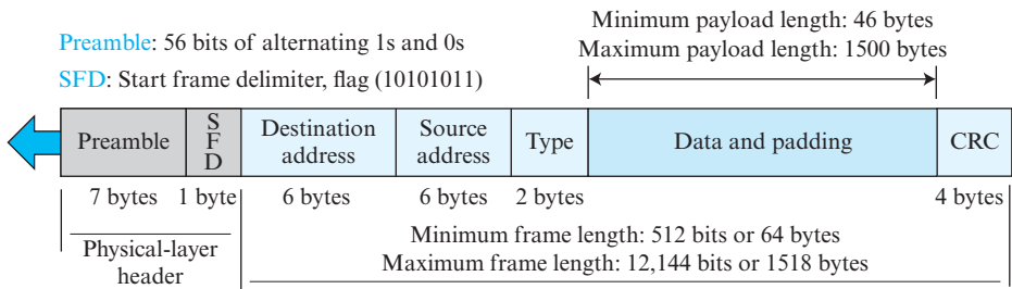
Figure 5.55 Ethernet frame
