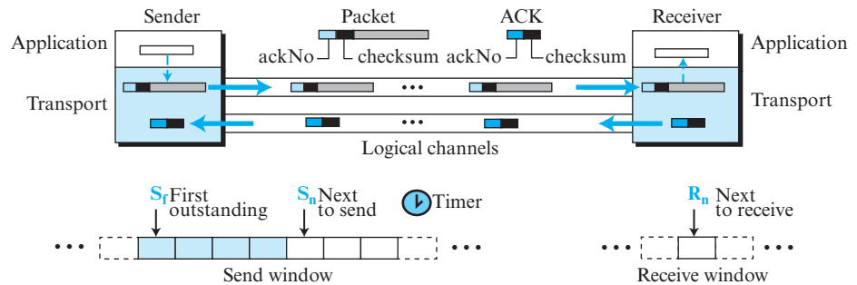
Figure 3.23 Go-Back-N protocol
