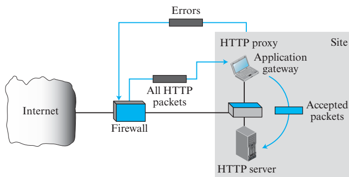
Figure 10.62 Proxy firewall
