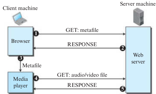
Figure 8.25 Using a Web server with a metafile
