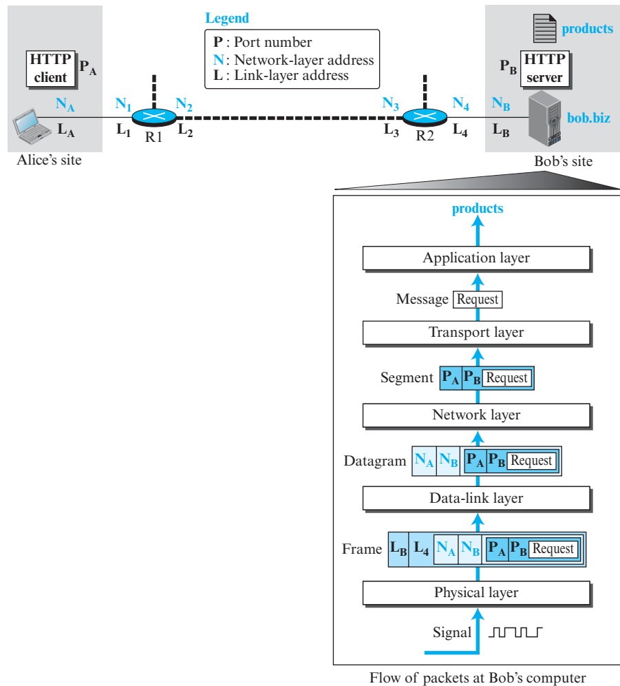
Figure 5.53 Activities at Bob's site
