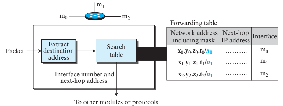
Figure 4.45 Simplified forwarding module in classless address
