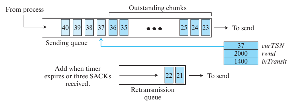
Figure 8.57 Error control, sender site
