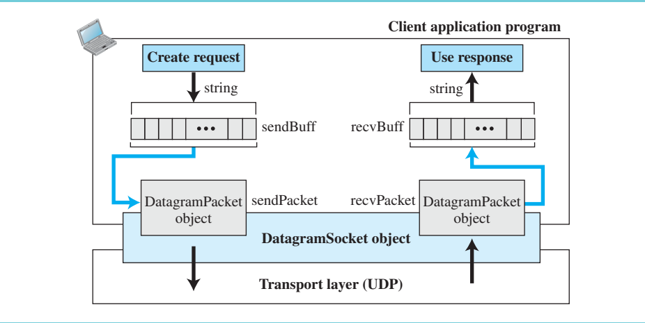
Figure 11.2 Design of the UDP Client
