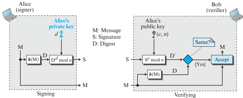
Figure 10.21 The RSA signature on the message digest
