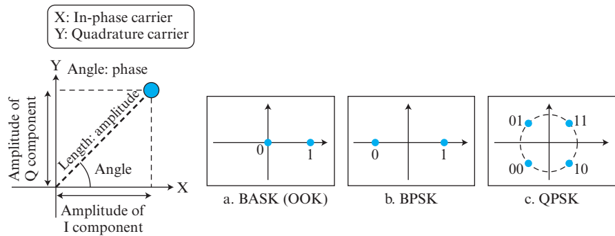
Figure 7.39 Concept of a constellation diagram
