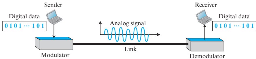
Figure 7.35 Digital-to-analog conversion
