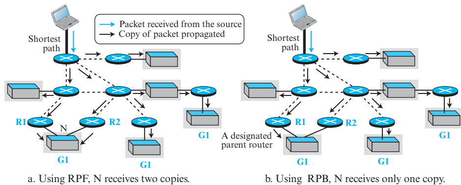
Figure 4.96 RPF versus RPB
