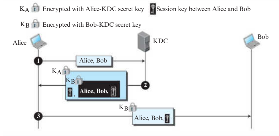
Figure 10.26 Creating a session key using KDC
