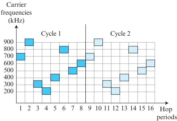
Figure 7.55 FHSS cycles
