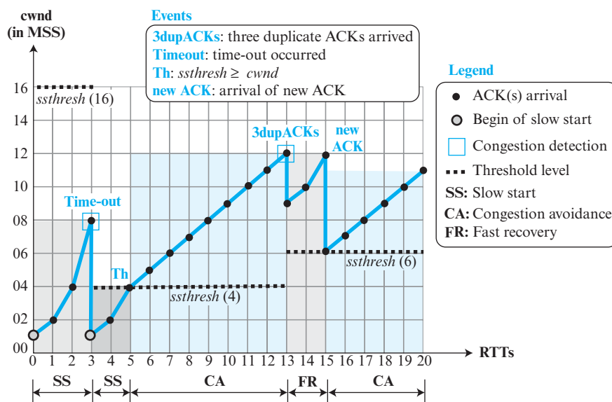
Figure 3.71 Example of a Reno TCP
