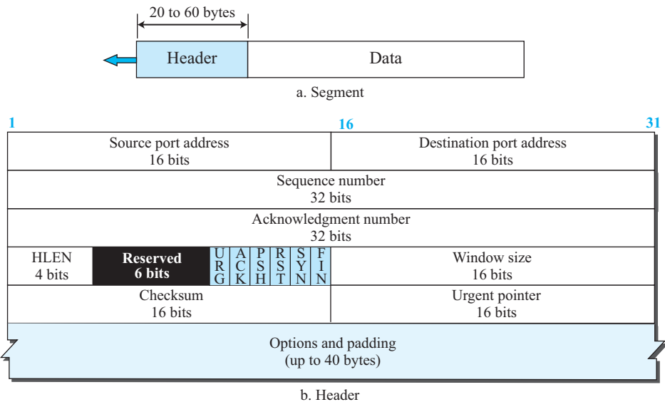
Figure 3.44 TCP segment format
