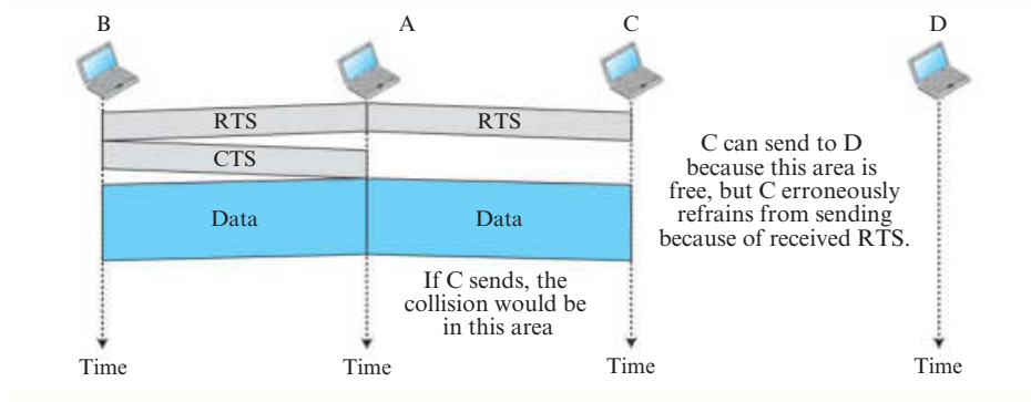
Figure 6.14 Exposed station problem
