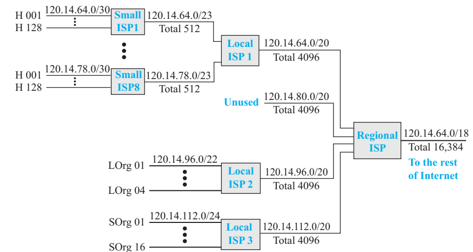
Figure 4.49 Hierarchical routing with ISPs
