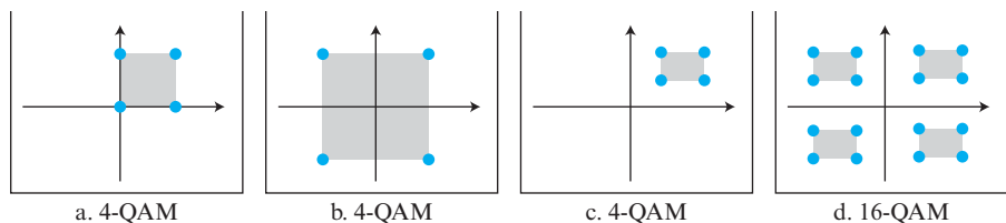
Figure 7.40 Constellation diagrams for some QAMs
