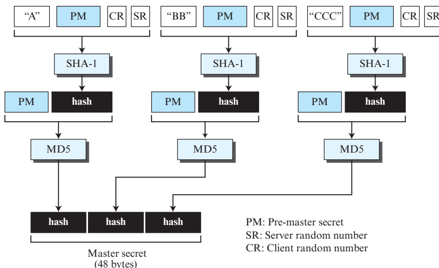
Figure 10.40 Calculation of master secret from pre-master secret
