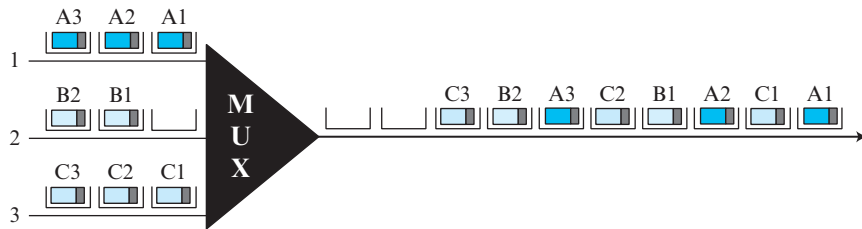
Figure 5.76 ATM multiplexing
