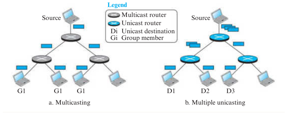
Figure 4.89 Multicasting versus multiple unicasting
