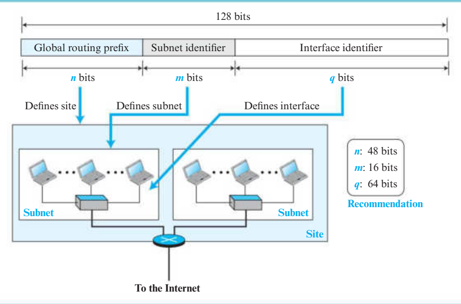
Figure 4.103 Global unicast address
