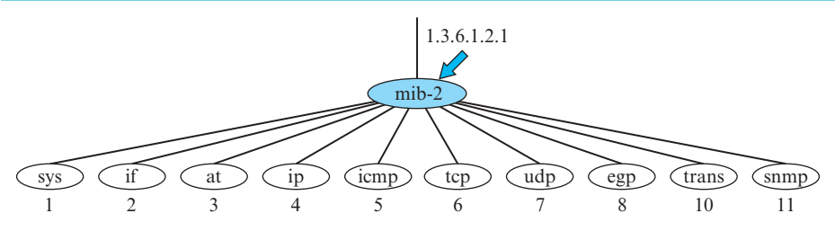
Figure 9.13 Some mib-2 groups
