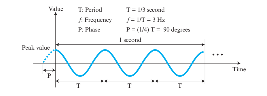
Figure 7.3 A sine wave
