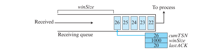
Figure 8.54 Flow control, receiver site
