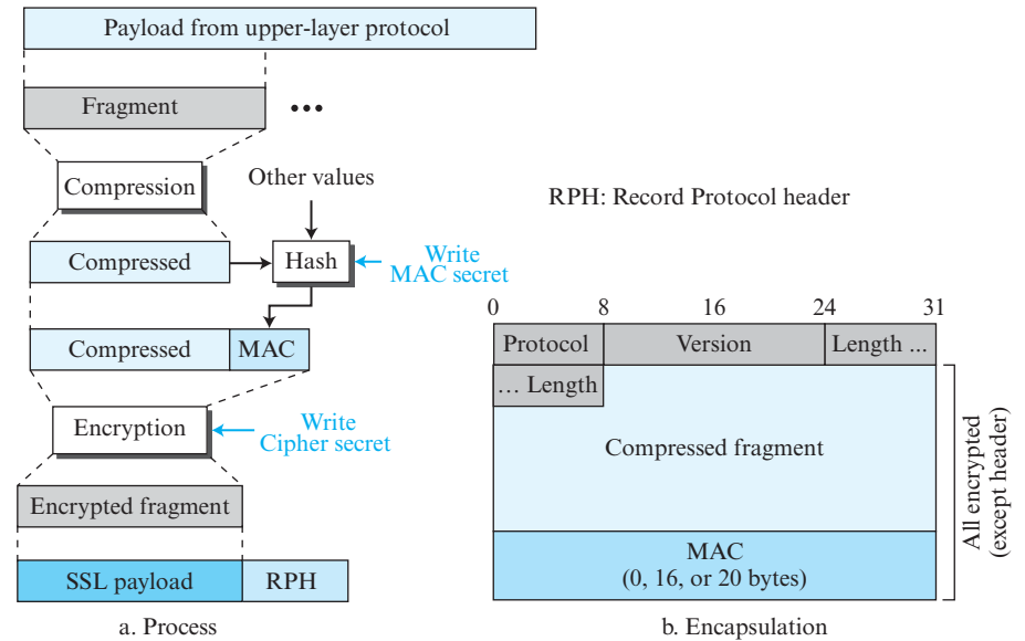
Figure 10.45 Processing done by the Record Protocol
