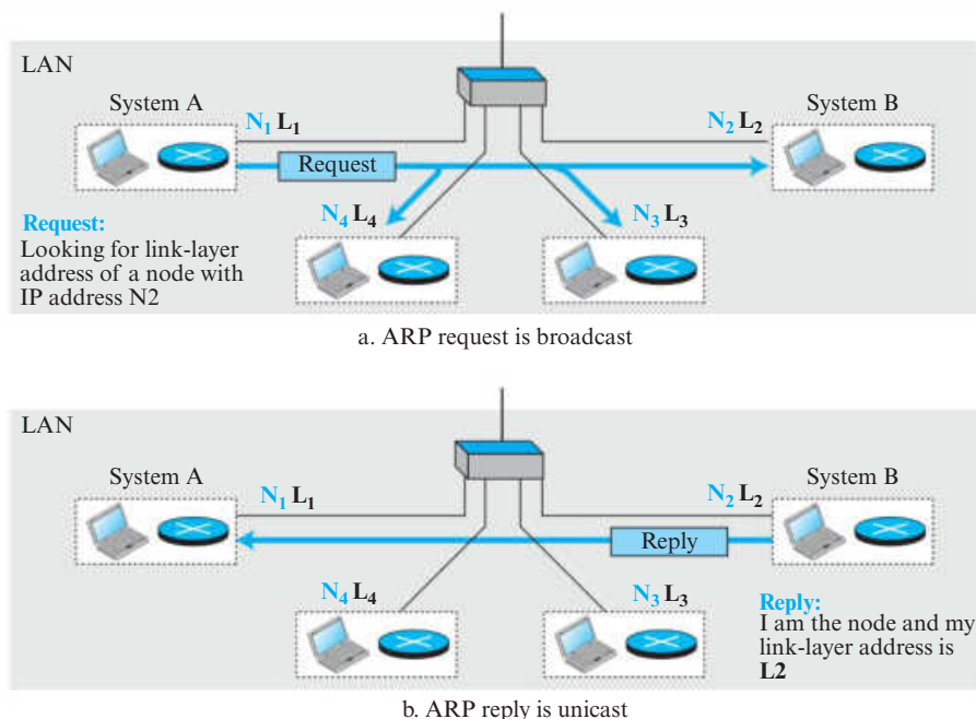
Figure 5.47 ARP operation
