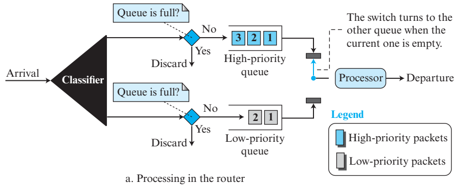
Figure 8.60 Priority queuing
