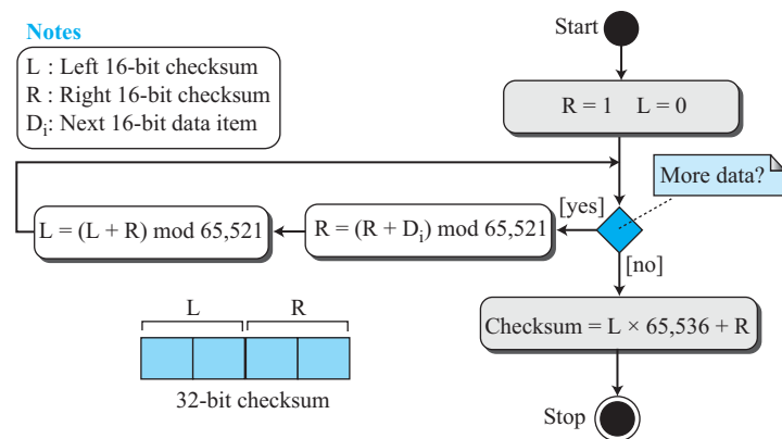
Figure 5.19 Algorithm to calculate an Adler checksum
