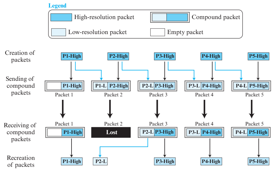
Figure 8.34 Compounding high- and low-resolution packets
