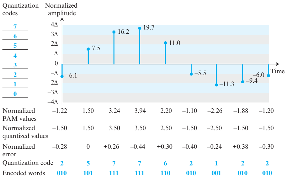
Figure 7.32 Quantization and encoding of a sampled signal
