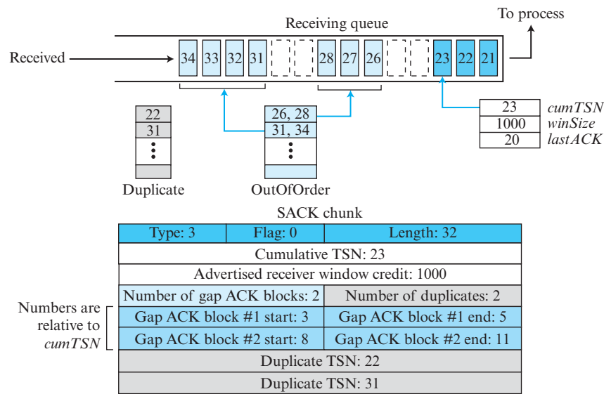
Figure 8.56 Error control, receiver site
