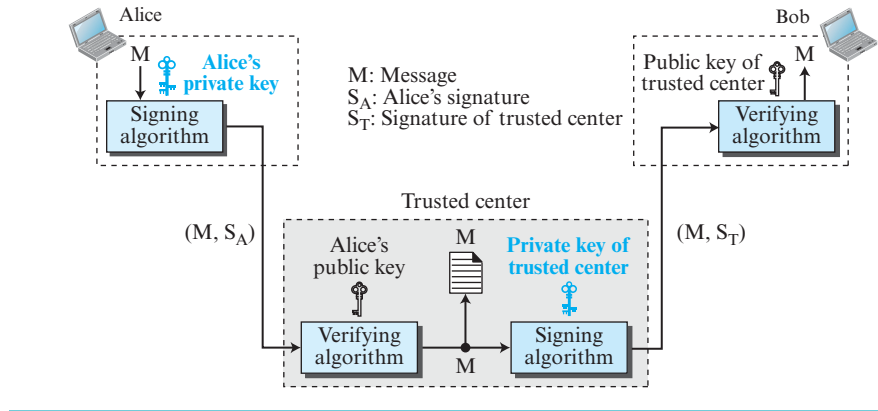
Figure 10.20 Using a trusted center for non-repudiation
