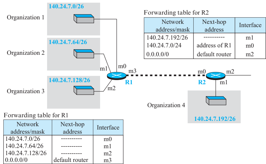
Figure 4.48 Longest mask matching
