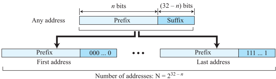
Figure 4.34 Information extraction in classless addressing
