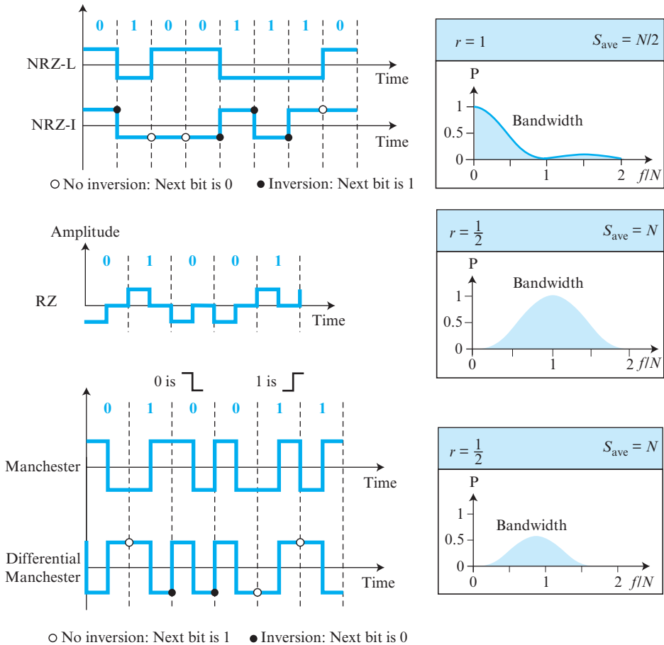
Figure 7.20 Polar schemes
