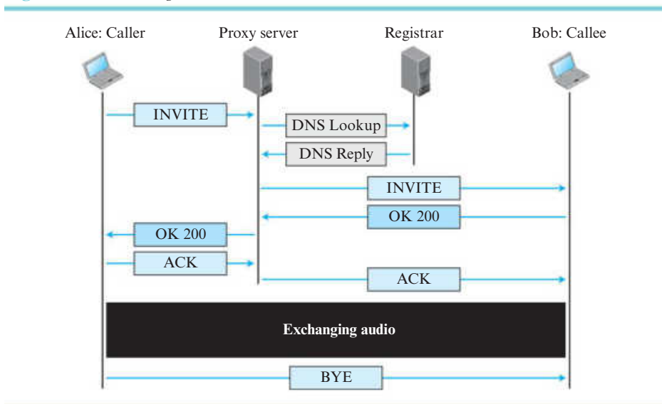
Figure 8.41 Tracking the callee
