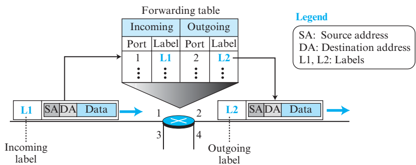
Figure 4.6 Forwarding process in a router when used in a virtual-circuit network
