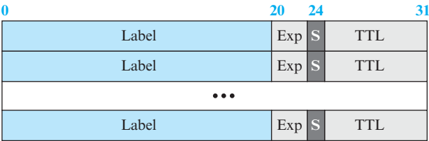
Figure 4.53 MPLS header made of a stack of labels
