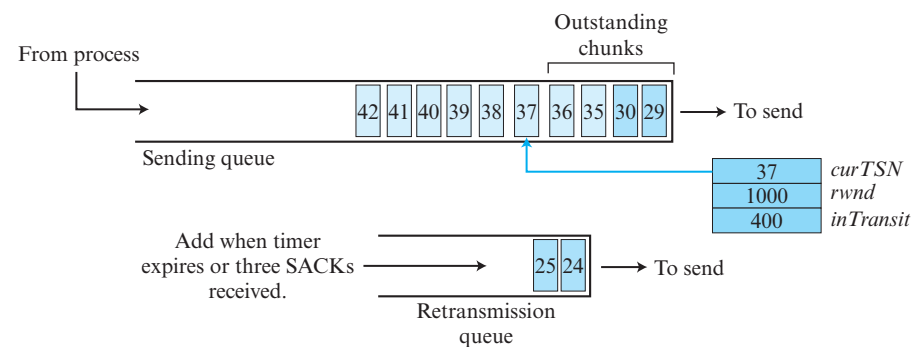
Figure 8.58 New state at the sender site after receiving a SACK chunk
