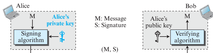
Figure 10.18 Digital signature process
