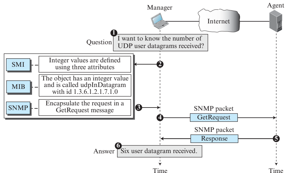
Figure 9.5 Management overview
