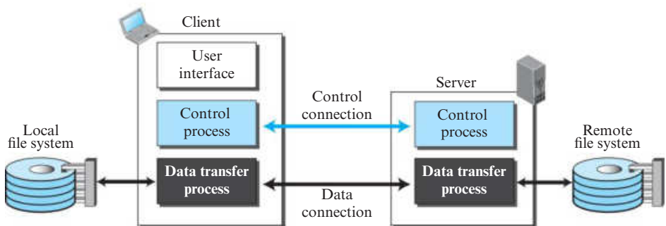
Figure 2.17 FTP
