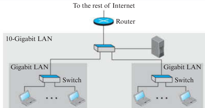
Figure 5.87 Routing example
