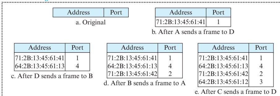
Figure 5.86 Learning switch
