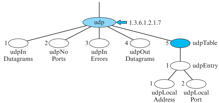
Figure 9.14 udp group
