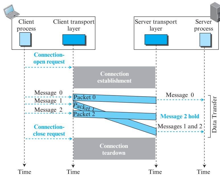
Figure 3.15 Connection-oriented service
