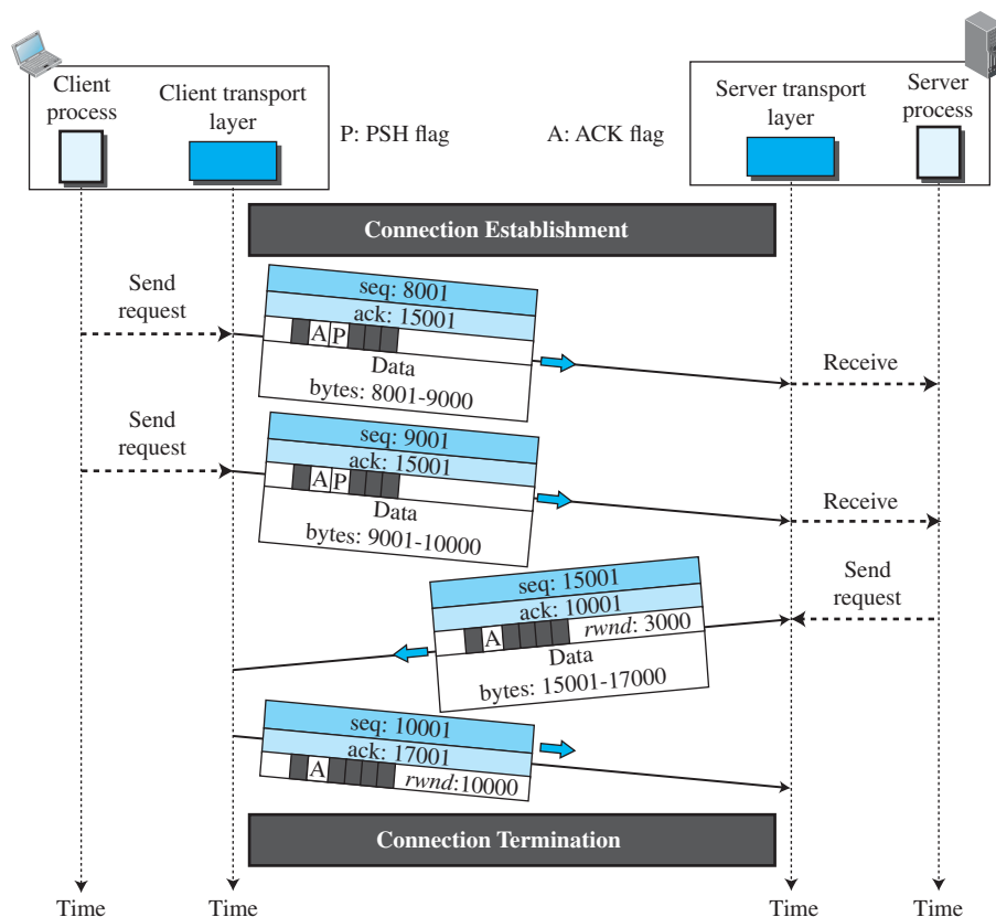
Figure 3.48 Data transfer
