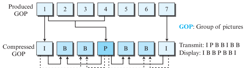
Figure 8.22 MPEG frames
