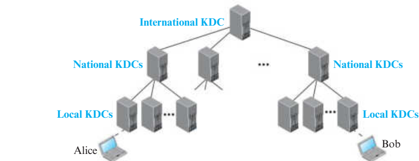
Figure 10.25 Multiple KDCs
