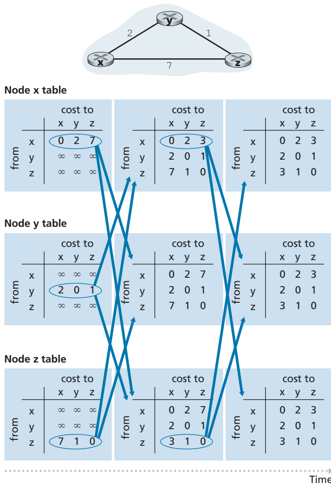
Figure 5.6 ♦ Distance-vector (DV) algorithm in operation
