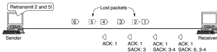
Figure 6-48. Selective acknowledgements.
