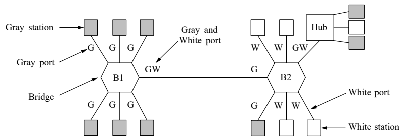
Figure 4-39. Two VLANs, gray and white, on a bridged LAN.
