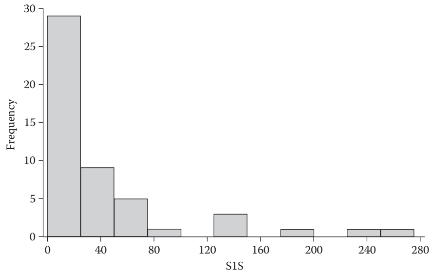
Figure 5.1 Histogram of squared residuals from Eq. (5.1).
