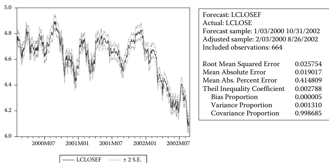
Figure 16.5 Actual and forecast IBM prices.
