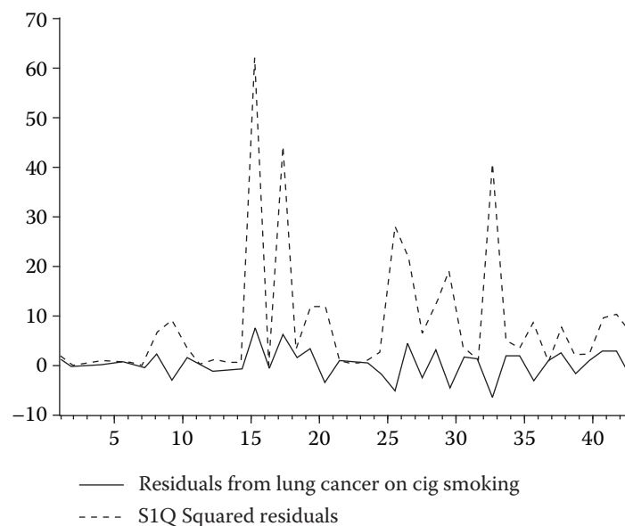
Figure 7.1 Residuals and squared residuals of regression in Table 7.9.
