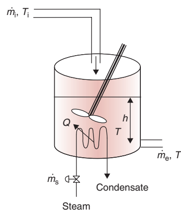
■ Figure 3.19 A tank of water heated with an indirect steam heat exchanger.
