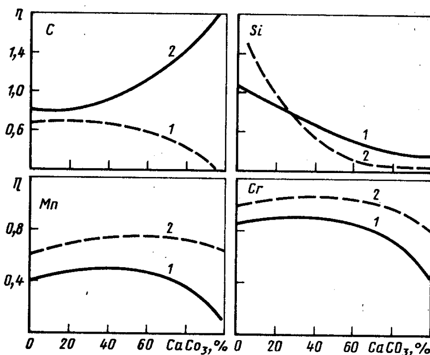
5.10-rasm. Qoplamali elektrodlar bilan payvandlashda \text{CaCO}_3/\text{F}_2 nisbat turlicha bo'lganda \text{CaCO}_3 - \text{F}_2 ( K_{\text{QM}} = 0,3 ) o'tish koeffitsientlari: 1 - CB-18ГCA markali simdan tayyorlangan sterjen; 2 - CB-06X19H9T markali simdan ishlangan sterjen
