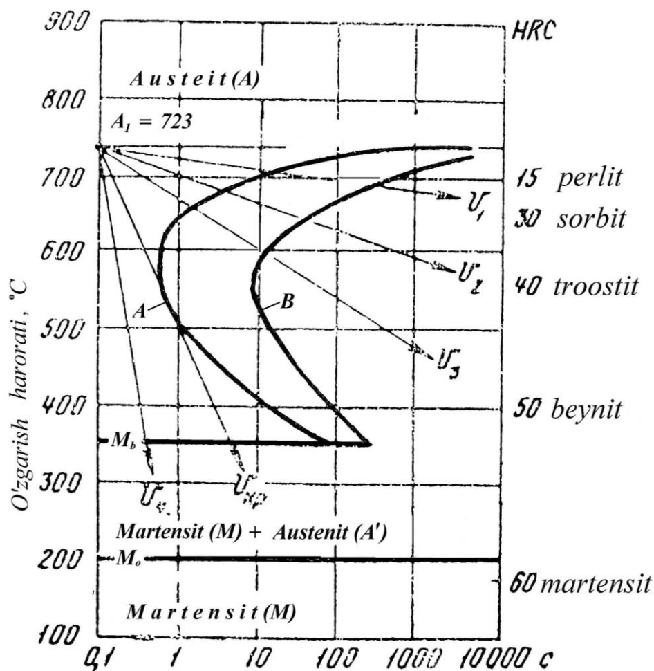
1.1-rasm. Kam uglerodli po‘lat austenitining izotermik (o‘zgarmas haroratda) parchalanish diagrammasi:
