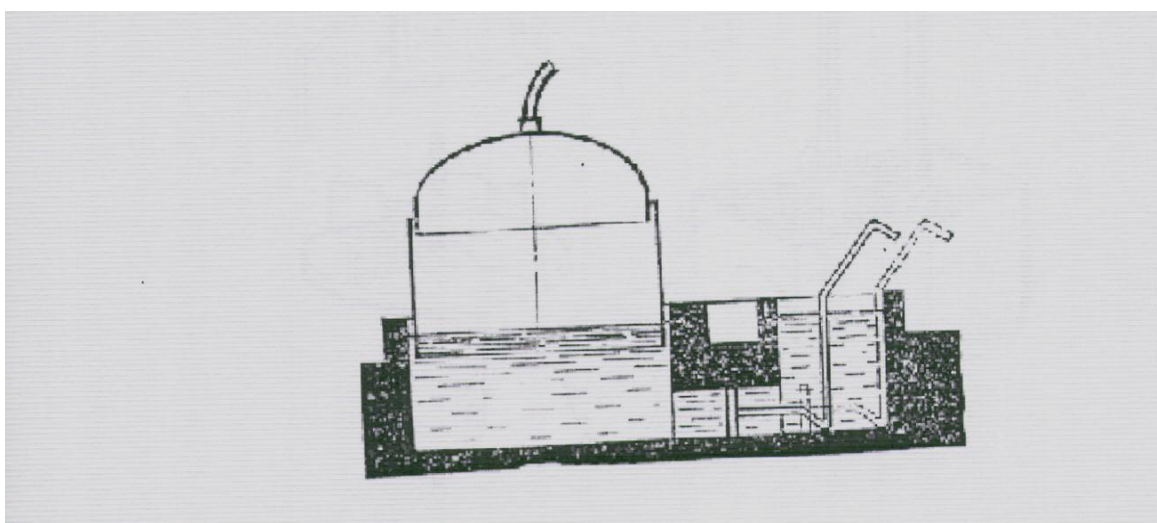
26-rasm. Biogaz olish uchun bochkasimon qurilma
