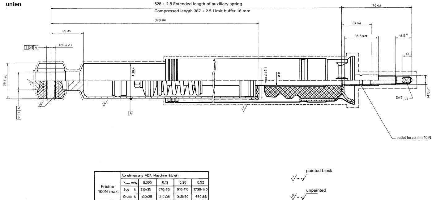
Fig. 5.31 After an original drawing by Bilstein of the front axle damper of the Mercedes Benz C (1997) class with a stroke of s_D = 141 mm, the fixed length L_{fix} = 246 mm, pin-type joint at the top (with a crimped spacer) and eye-type joint at the bottom; the piston rod comes out at the top. The supplementary spring shown on the right is surrounded by a short, stable tube and comes into contact with this and the support disc located above the piston rod guide when the spring compresses. The tube also carries the actual plastic sleeve, which reaches up to the damper centre.
