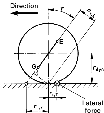
Fig. 3.121 Due to the tyre caster r_{T,T} , which is always present during cornering, the lateral force lever is extended and becomes (Fig. 2.50)
