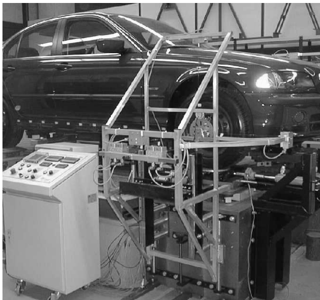
Fig. 3.163 Elastokinematics test stand of the Chassis/Simulation Technology Lab-oratory of the University of Applied Science, Cologne. The movements of the wheels are measured by a combined system of filament potentiometers and inclinometers constructed on the basis of a system of error and fault minimization; forces are measured by means of force transducers. A computer system is used for measurement, stipulation of the required values and evaluation. Forces can be applied with the normal tyres left in place or via wheel replacement carriers; air-sprung sliding plates are used to minimize friction.
