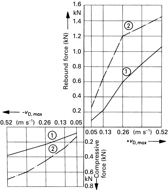
Fig. 5.43 Rear axle damping curve; 1 is the standard setting and 2 that for the heavy-duty version.
