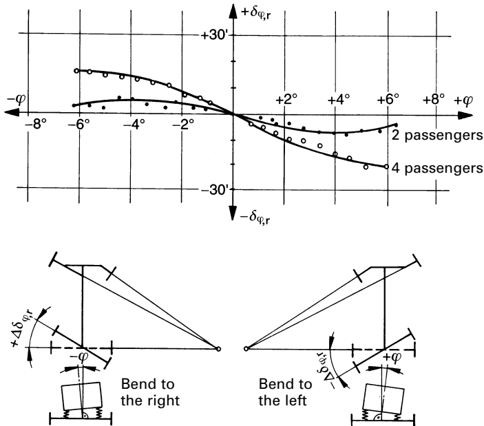
Fig. 3.77 Angled position by the angle \Delta\delta_{\varphi,r} as a function of the roll angle \varphi measured on the driven rigid rear axle of a conventional passenger car occupied with two and four people. When there are two people in the vehicle and \varphi = 4^\circ , \Delta\delta_{\varphi,r} = 6' . The body roll-steering factor would then be \Delta\delta_{\varphi,r}/\Delta\varphi = 0.1^\circ/4^\circ = 0.025 .
