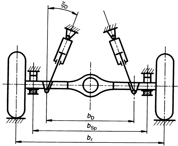
Fig. 5.23 If the dampers are fixed to a rigid axle at an angle, the angle \xi_D increases with compression with the advantage of a more unfavourable damping in the loaded condition. Moreover, the further in the dampers are positioned, the less they prevent the body roll movement.
