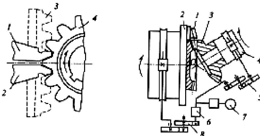
9.10-rasm. To'g'ri tishli konussimon g'ildirakka ishlov berish sxemasi:
