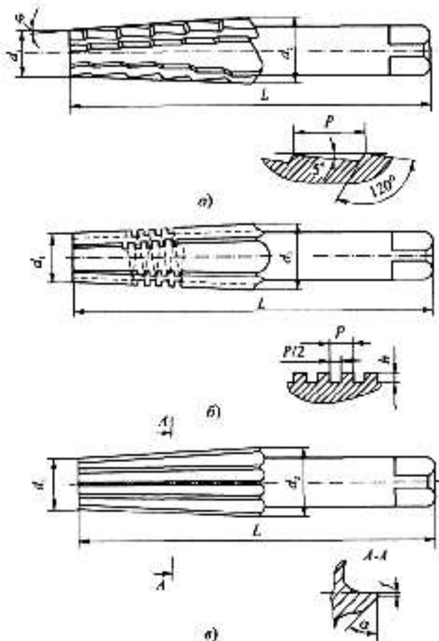
5.6-rasm. Konusli razvyortkalar jamlamasi: a – dastlabki (№1); b – oraliq (№2); v – toza (№3)
