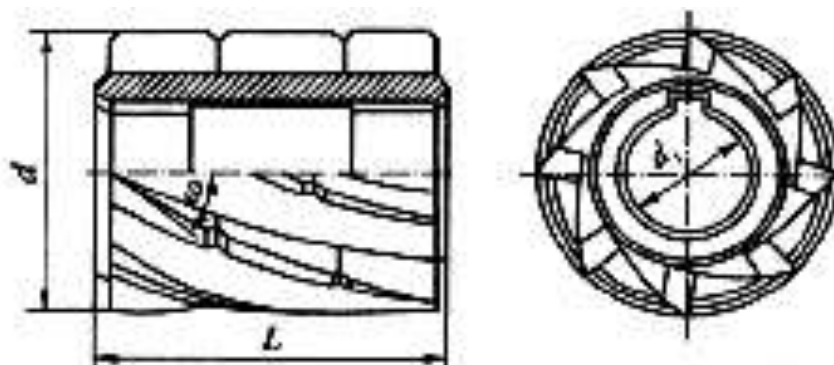
6.8-rasm. Kavsharlangan qattiq qotishmali plastinalar bilan jihozlangan tsilindrsimon freza
