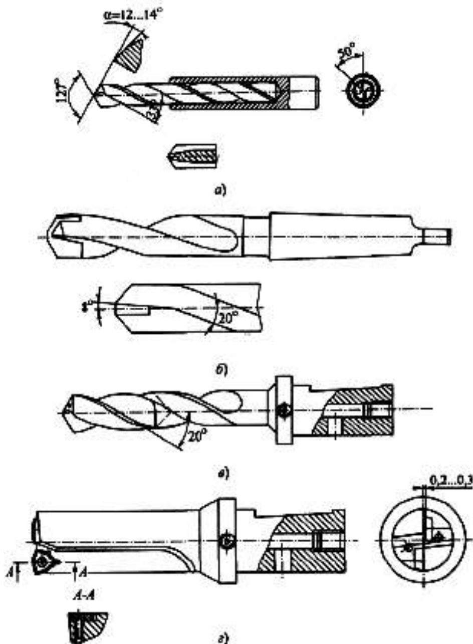
3.8-rasm. Qattiq qotishmali parmalar:
