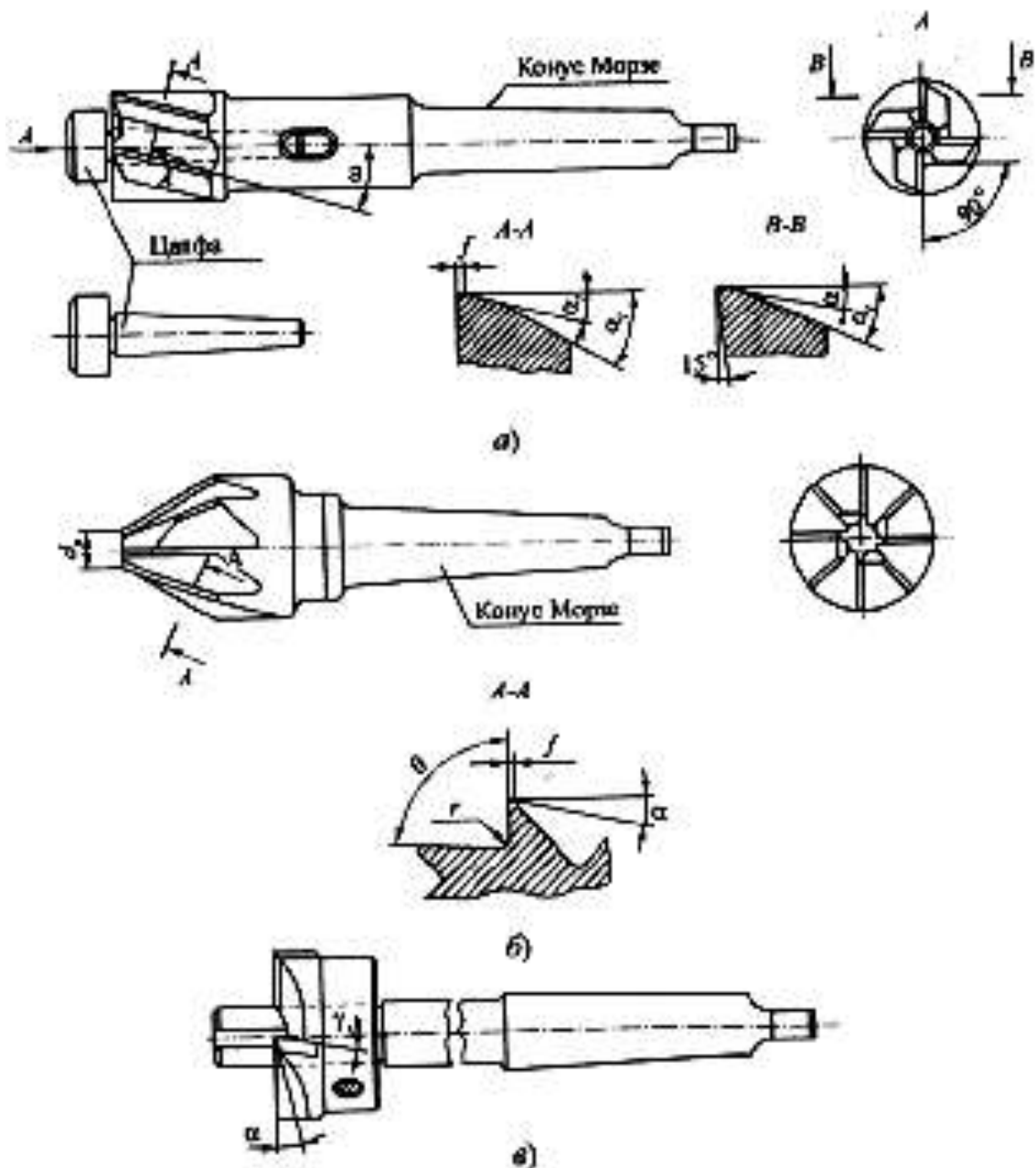
4.9-rasm. Zenkovkalar:
