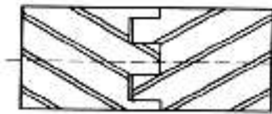
6.2-rasm. Tishlarining yo'nalishi turlicha bo'lgan yig'ma freza
